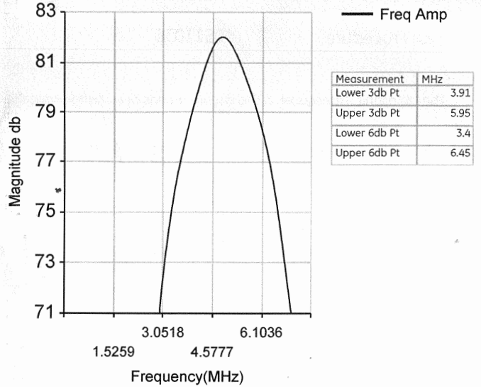
Frequency Spectrum
