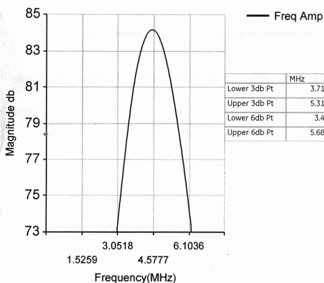
Frequency Spectrum
